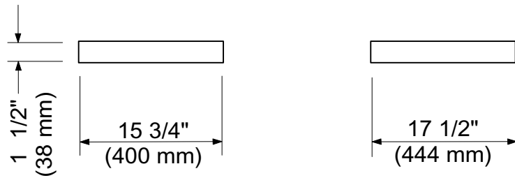
SCALE BASE
